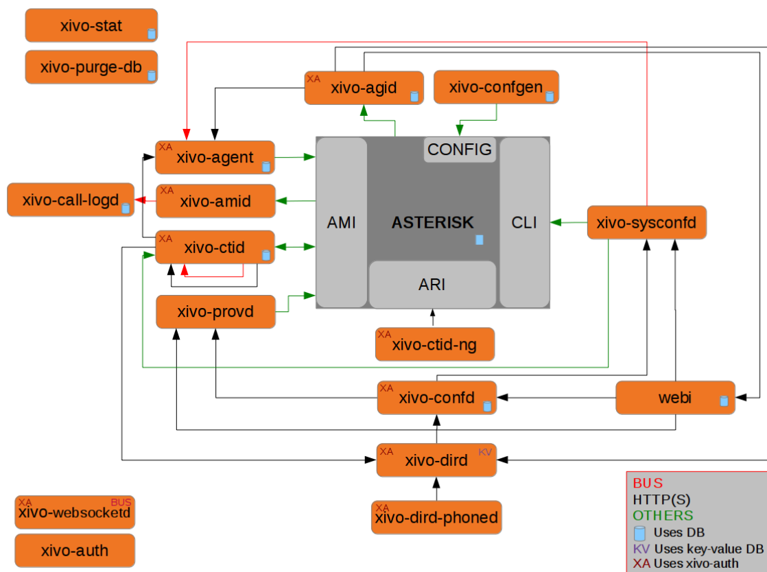
Fig. 1.105: Relationships between the components of XiVO. (source)
