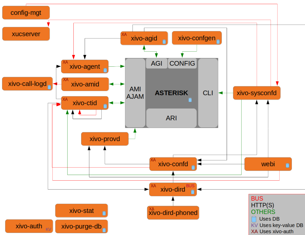
Fig. 1: Relationships between the components of XiVO. (source)
