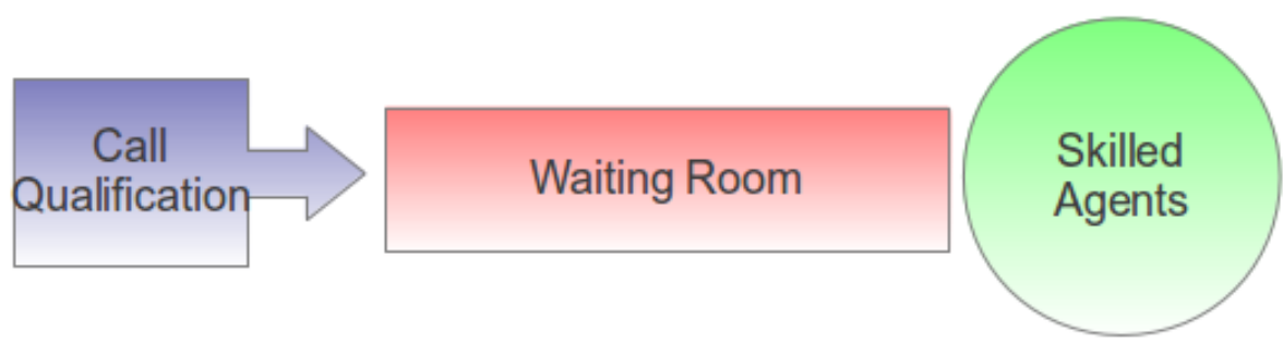
Fig. 2: Skills-Based Routing
