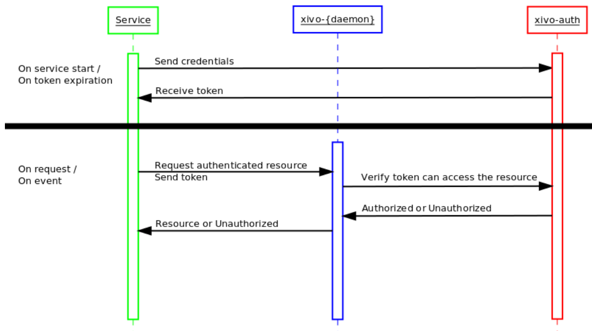
Fig. 12: Call flow of service authentication
